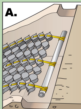
"Deadman" Pipe
