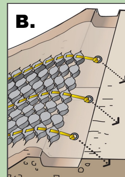
Earth anchors
